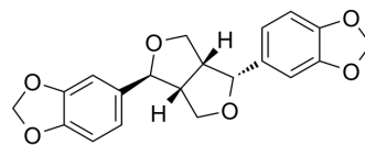
Relative stereochemistry.
