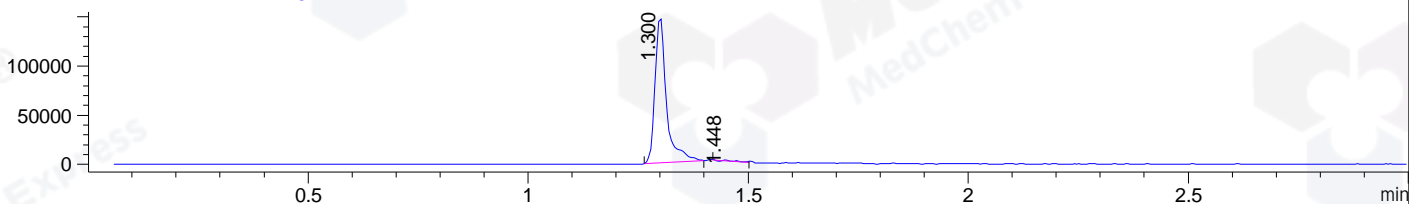
Ion 421, MSD1 421, Target Mass 420 +H Positive, EIC=420.7:421.7
