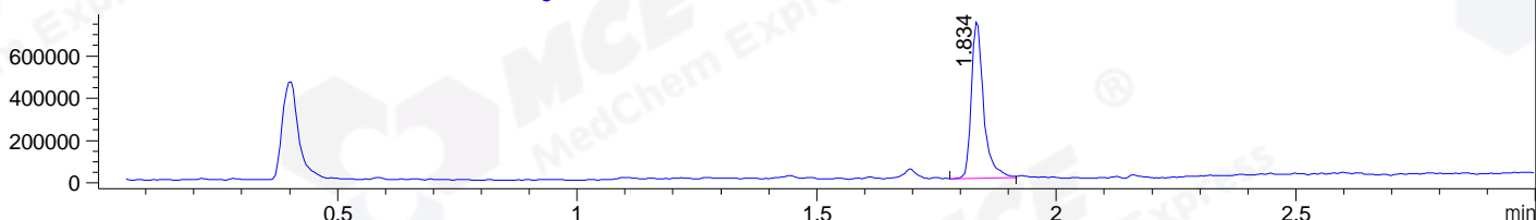
Ion 651, MSD1 651, Target Mass 650 +H Positive, EIC=650.7:651.7
