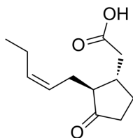
Relative stereochemistry
