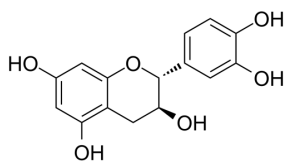
Relative stereochemistry
