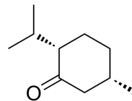
Relative stereochemistry
