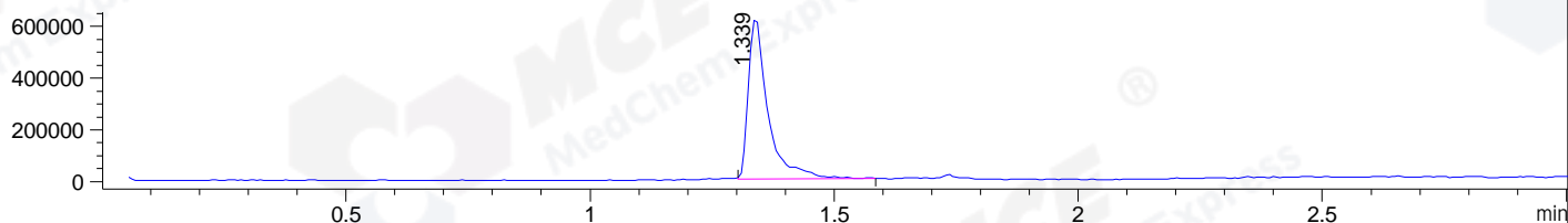
Ion 228.3, MSD1 228.3, Target Mass 227.3 +H Positive, EIC=228:229
