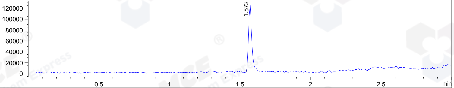
Ion 219, MSD1 219, Target Mass 218 +H Positive, EIC=218.7:219.7
